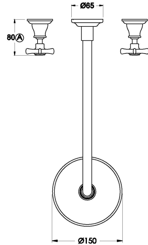
Top view:
