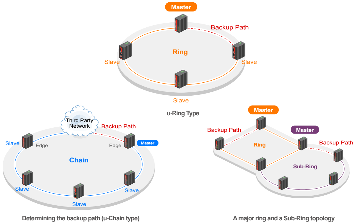
Figure 4 : u-Ring Type
