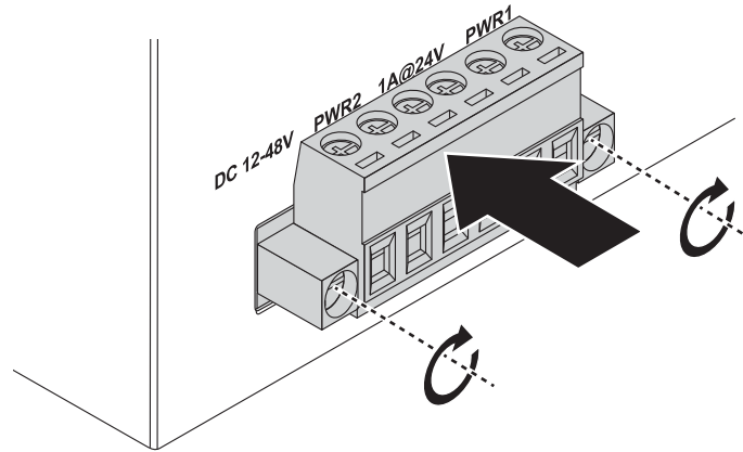
Figure 2.23 Securing a Terminal Block to a Receptor
