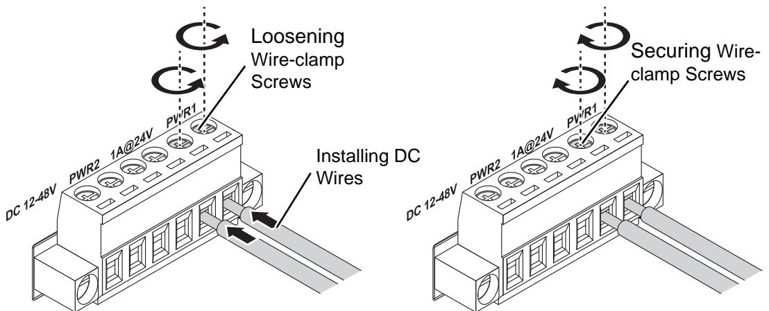
Figure 2.22 Installing DC Wires in a Terminal Block
