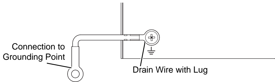
Figure 2.18 Grounding Connection
