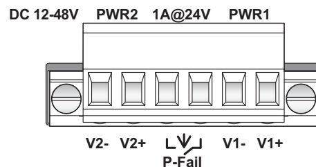
Figure 2.19 Terminal Receptor: Relay Contact
