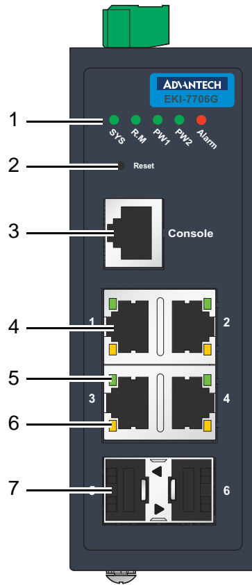
Figure 1.1 Front View
