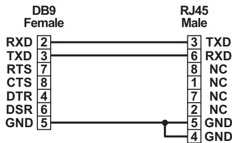
Figure 2.16 Pin Assignment
