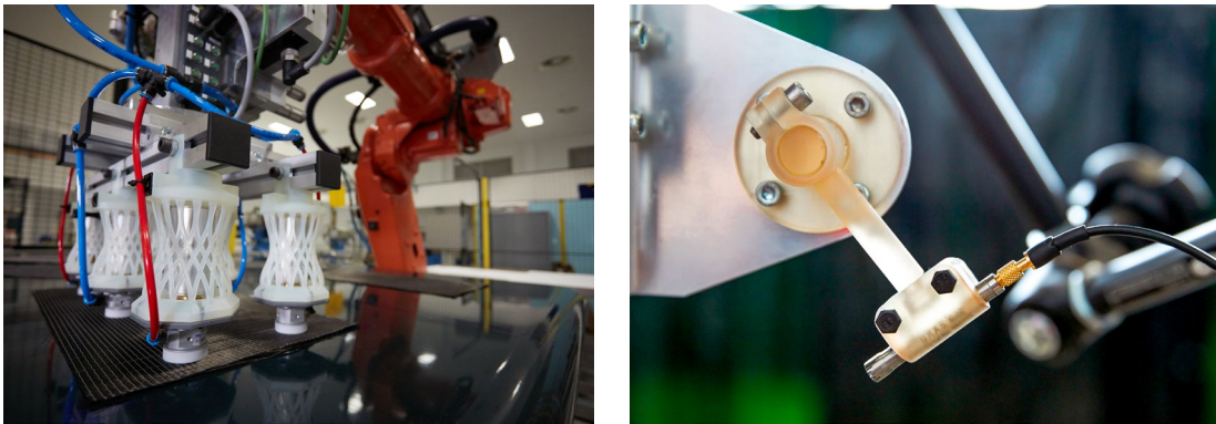
Engineers at AMRC use a fleet of 12 SLA 3D printers and a variety of engineering materials to print custom parts for diverse research projects, like brackets for a pick and place robot (left) and mounts for sensors in a high-temperature environment (right).
