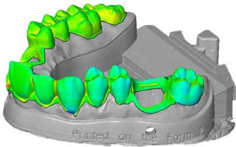
An example from the dental industry comparing a scanned component with the original CAD geometry, demonstrating the ability to maintain tight tolerances across an SLA printed part.
