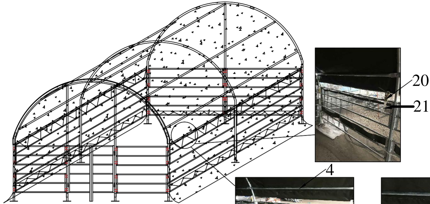
Figure 9 Fastening the Roof Cover
