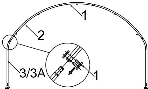
Figure 4 The arch installation
