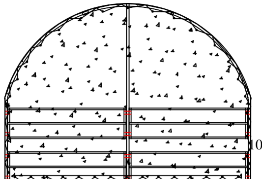
Figure 10 Installation of the Back Cover
