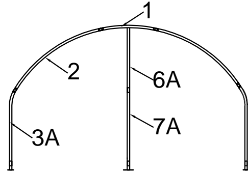
Figure 6 Frame Installation for Back Panel
