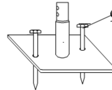
Figure 3 As Figure 3 shows, each baseflange is equipped with two stake pegs.
