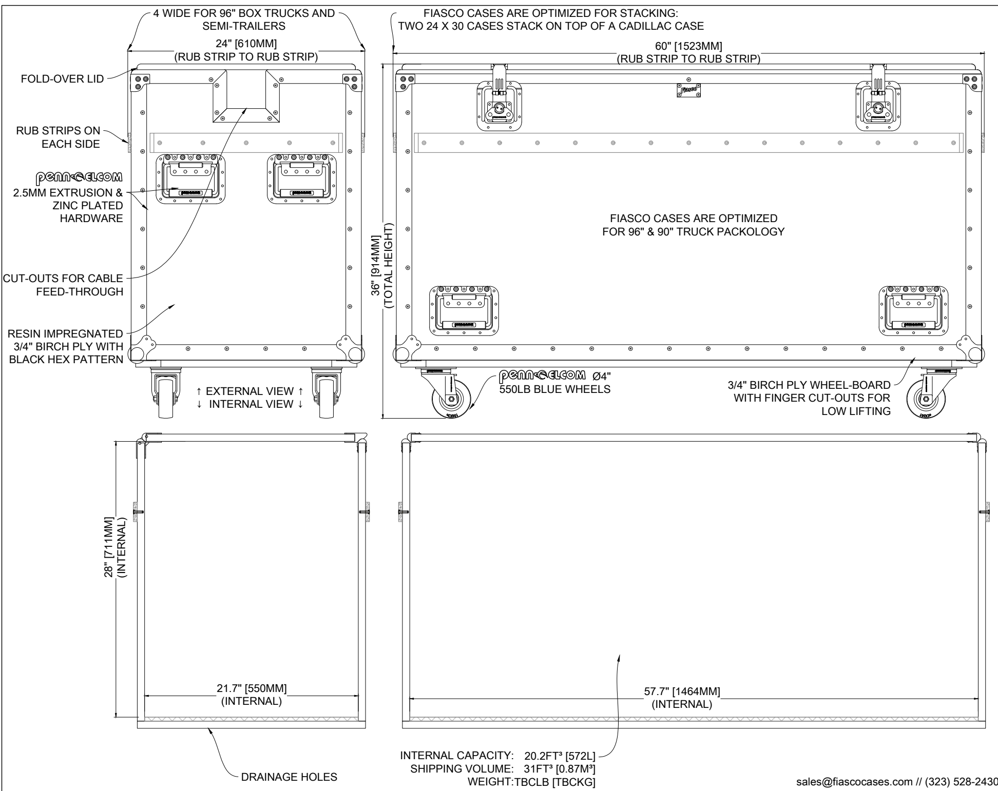
THIRD ANGLE PROJECTION
