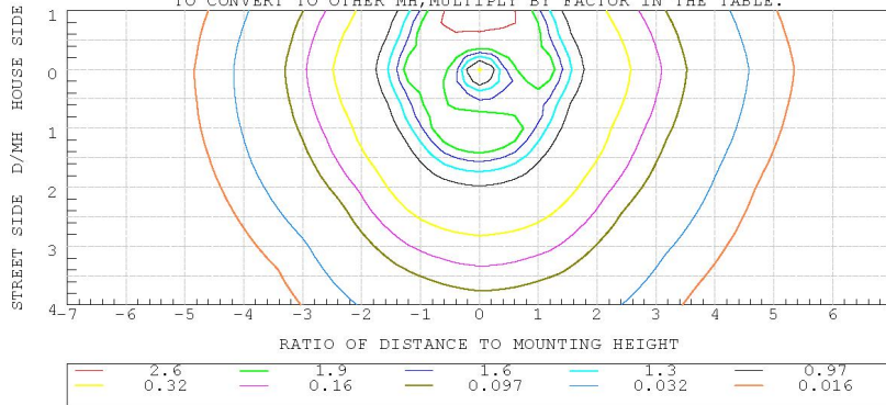
ROAD SURFACE ISOLUX DIAGRAM ILLUMINANCE AT MH=10 m, Enadir = 0.24 lx TO CONVERT TO OTHER MH, MULTIPLY BY FACTOR IN THE TABLE.
