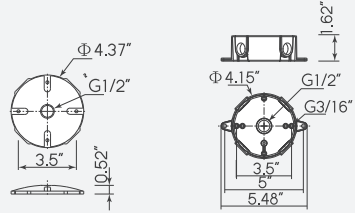
Weatherproof Cover
