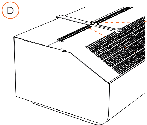
Fig. 6: Mounting with wall brackets
