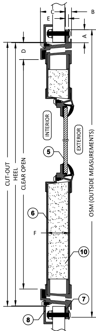
SECTION B-B
