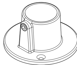
10x Base Plate D-131
