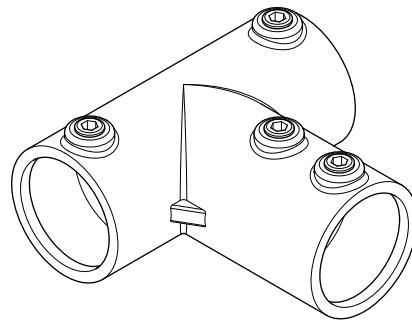
4x Extra Long Tee D-104L
