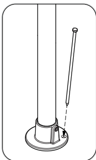
Base plate A & B
