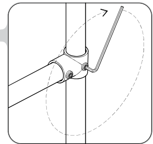
6. Tighten grub screw fixing the short tee to the swing leg tube.
