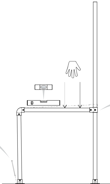
5. Push down on the twirly whirly bar until horizontal bar is level.
