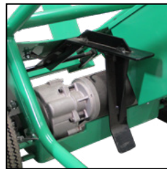
Foot Operated Trip Spring
