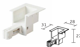
Microline Recessed End Feed
