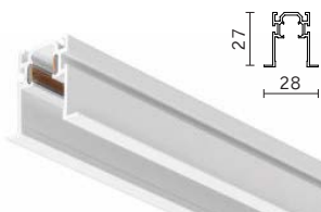
Microline Recessed Track - 2M
