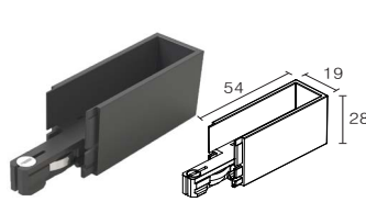
Microline End Feed
