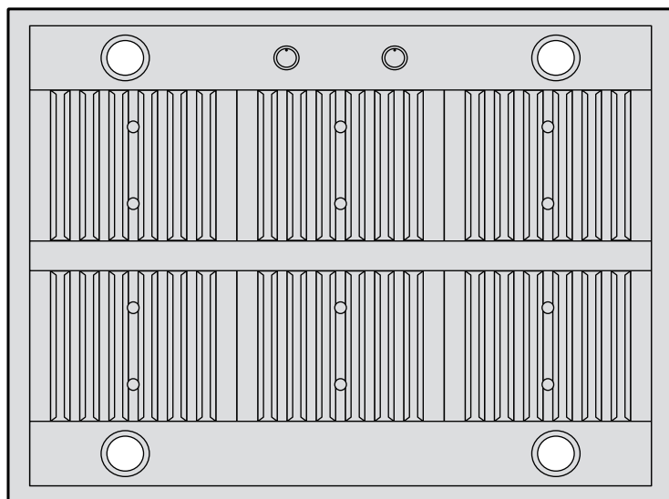
BOTTOM VIEW
