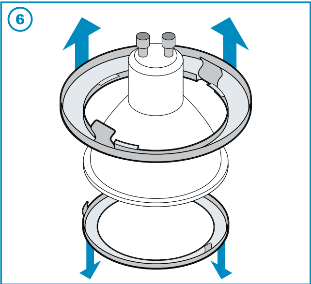
(Fig 6) Lift and remove outer ring. Remove inner ring from bulb. Replace GU10 bulb.
