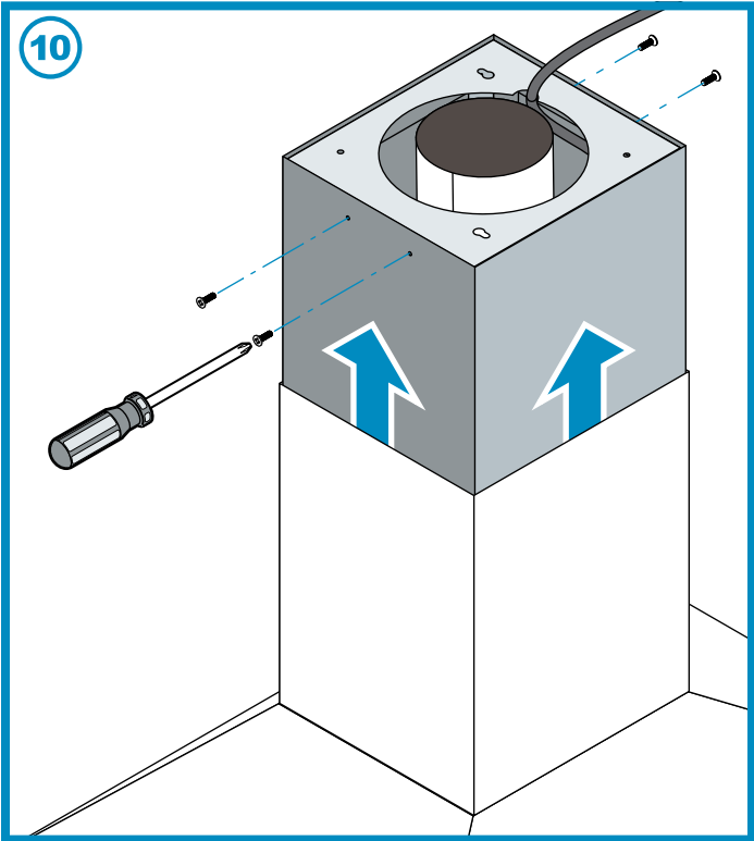
(Fig 10) Lift the inner sleeve of the chimney, and raise to the main frame. Fasten screws to each of the hole openings and ensure a secure fit.
