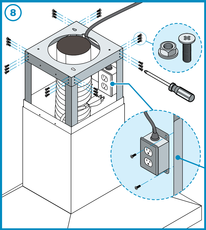
(Fig 8) Fasten arm extensions to the main frame with a screw on each side of each bracket with locking nut.
