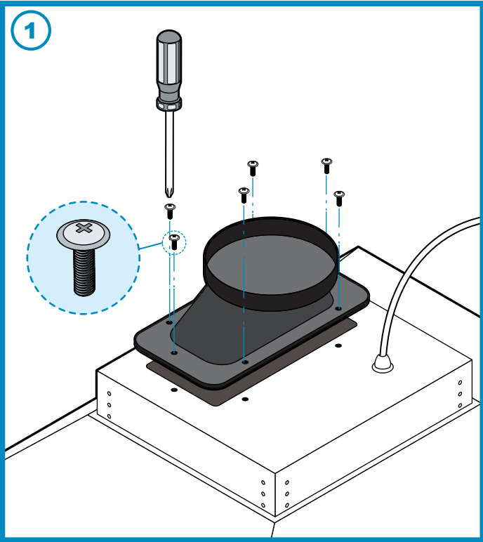
(Fig 1) Screw on 6"-Ø transition (8"-Ø optional) to the opening of the fan motor exit.
