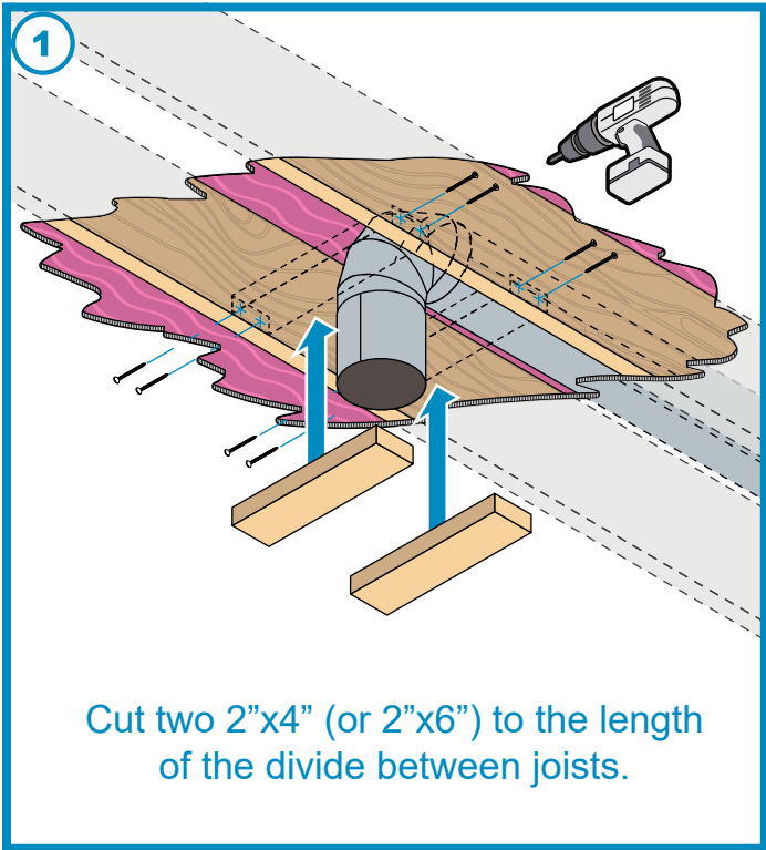
(Fig 1) Measure the main frame of the range hood support to the area planned for installation. Screw two 2"x4" onto joists as shown (woodscrews not included).
