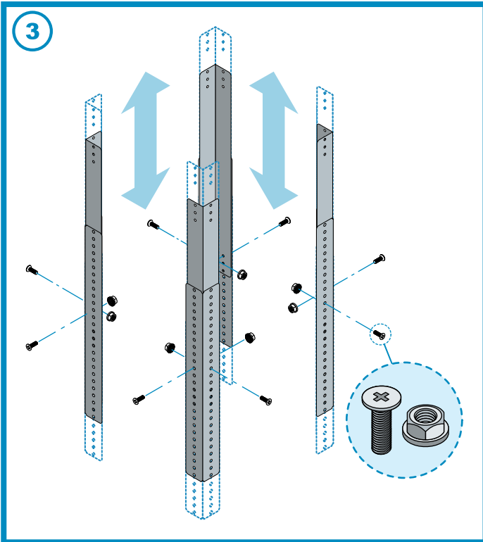
(Fig 3) Determine the height needed for the support extensions. Adjust length between the range of 17 ¾" to 29". Secure with 2 screws with locking nut each arm.
