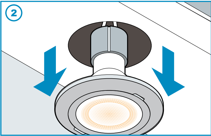
(Fig 1) Use a thin laminate card (like a business card, or plastic palette knife to produce scratches on the metal finish) and insert in between the switch panel and LED bulb housing. Work your way around (Fig 2) until the light housing pops out.
