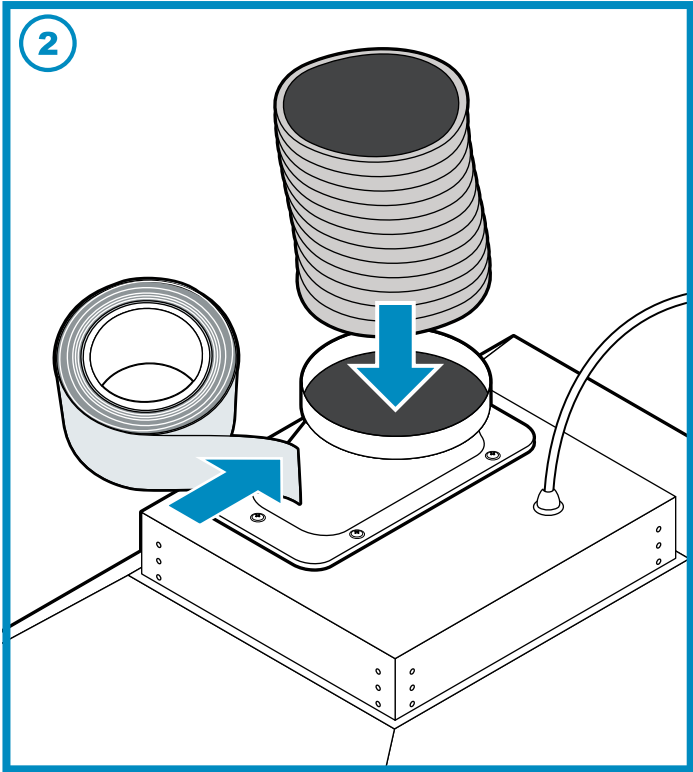
(Fig 2) Attach a flex duct (not included) to the transition. Use aluminum foil tape to secure a proper seal.
