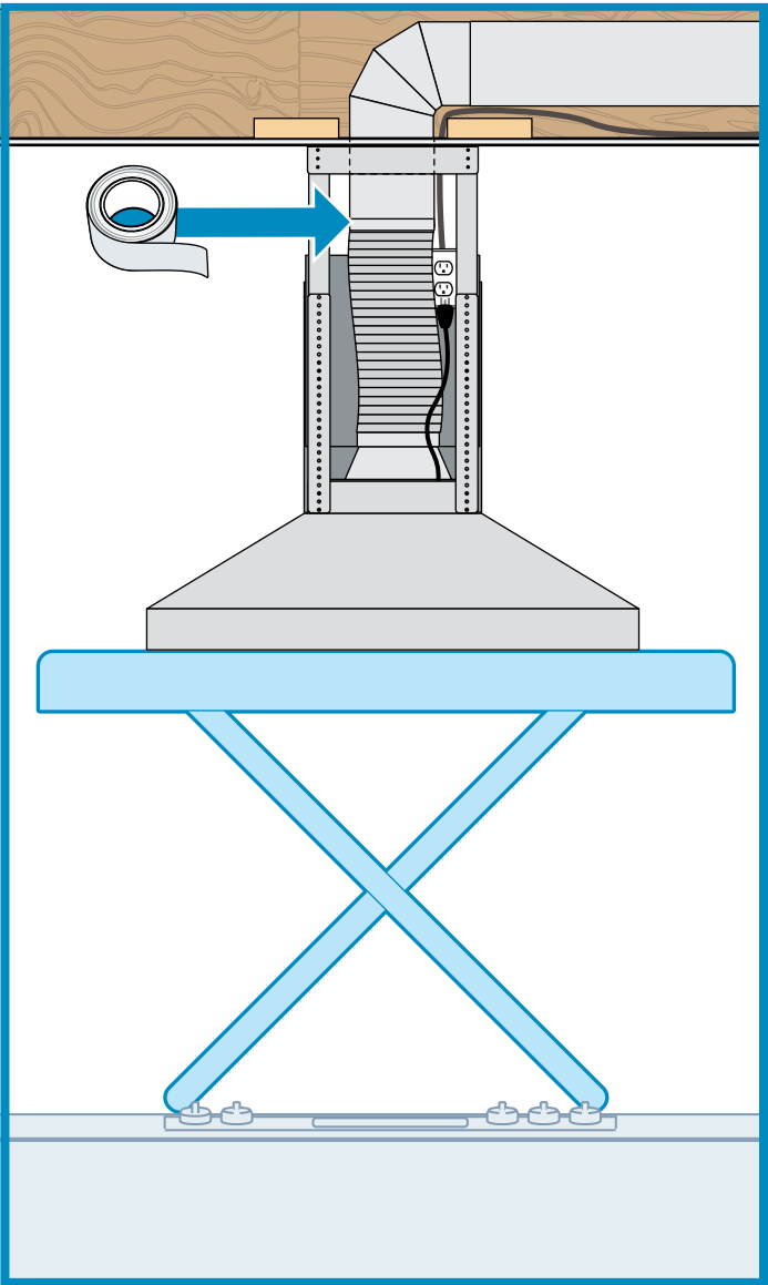
(Fig 7) Lift range hood and place arm extensions to the main frame attached to the ceiling. Connect the flex duct from the range hood to the ducting in the ceiling. Use aluminum foil tape to secure a proper seal.
