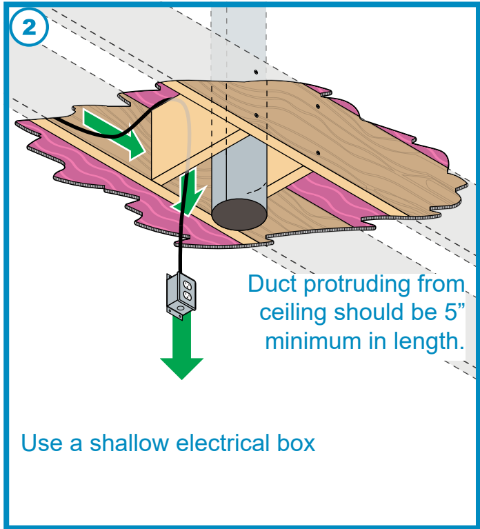
(Fig 2) Install an electrical outlet from the ceiling in between the braces. Use the 6"-Ø duct to the elbow connection (or use 8"-Ø if you are using the 10" transition).
