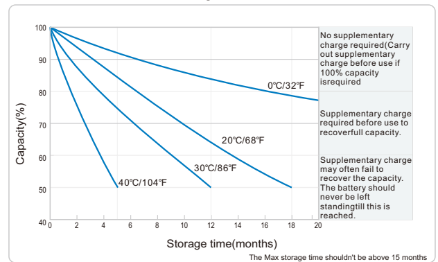
Self-discharge Characteristic
