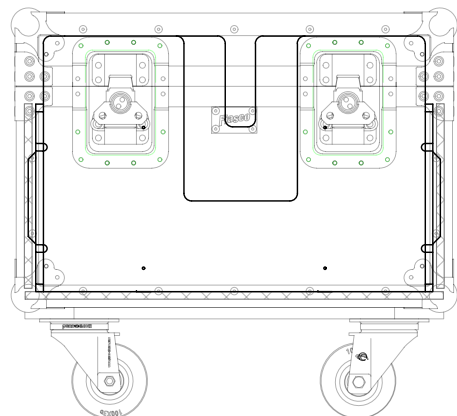
600 MOTOR INSERT INSTALLED IN 600 SHORT CASE
