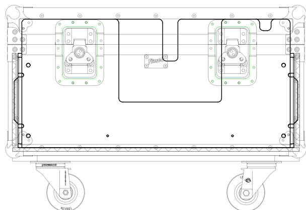
800 MOTOR INSERT INSTALLED IN 800 SHORT CASE
