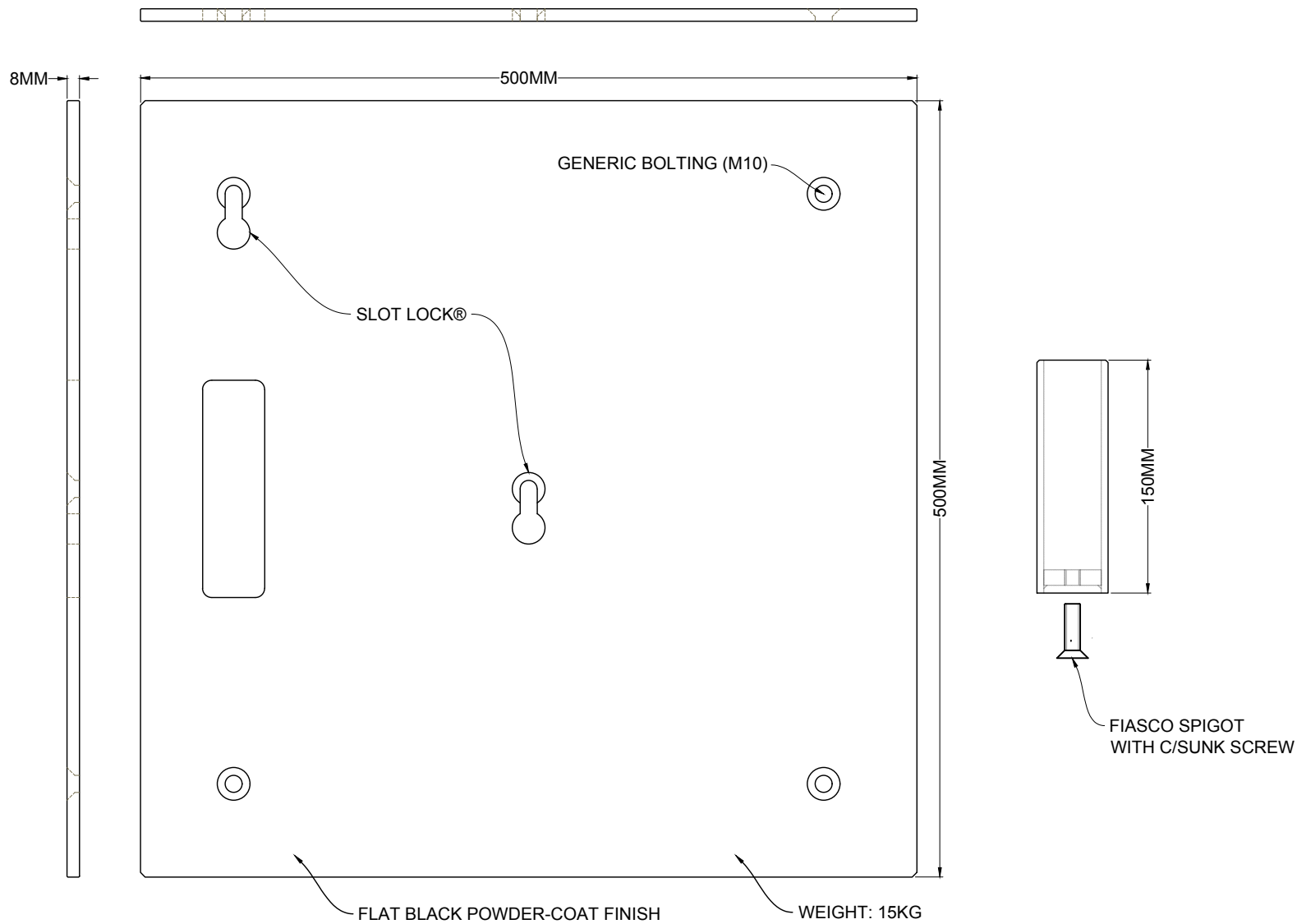
THIRD ANGLE PROJECTION
