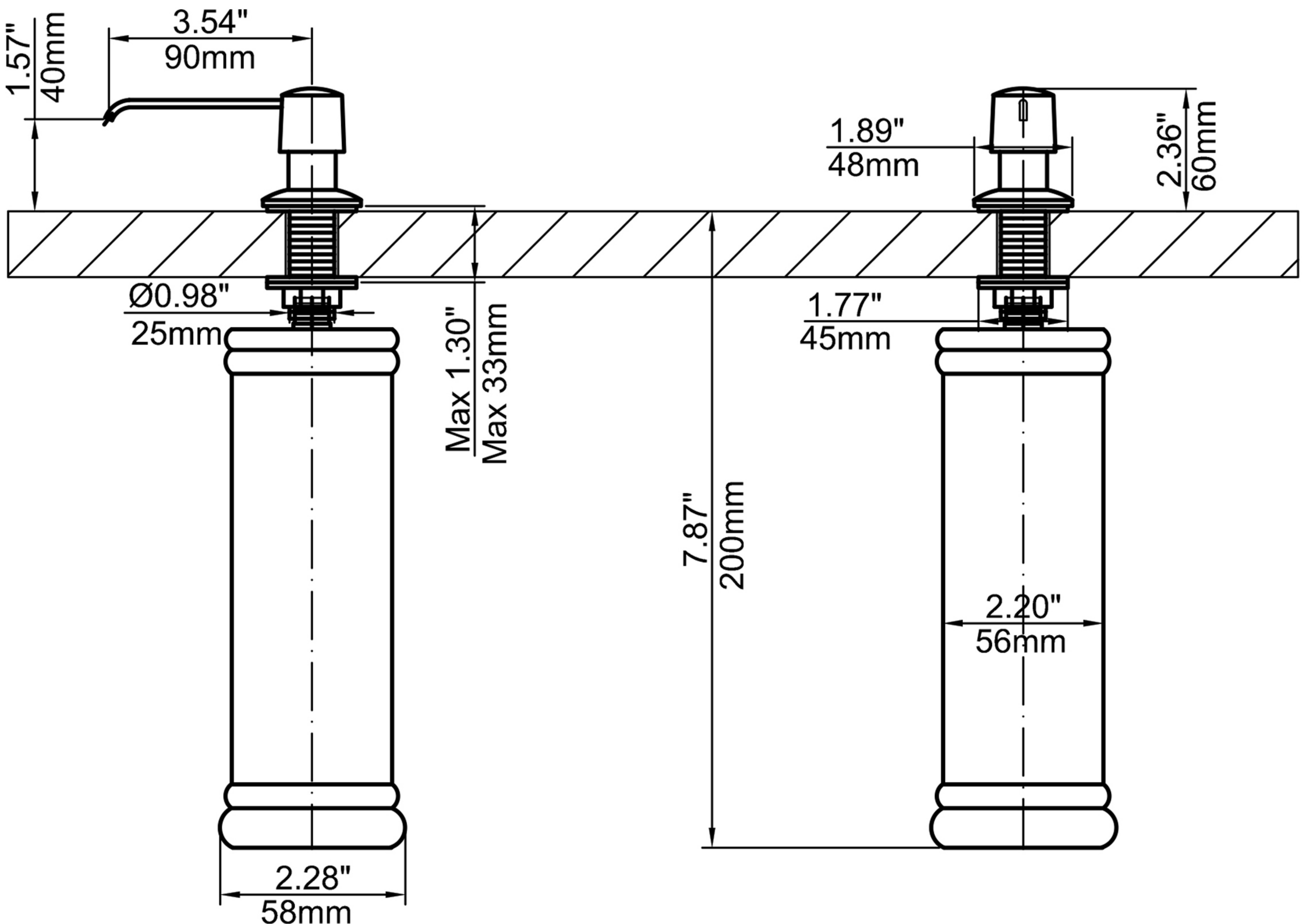
CRITICAL DIMENSIONS
