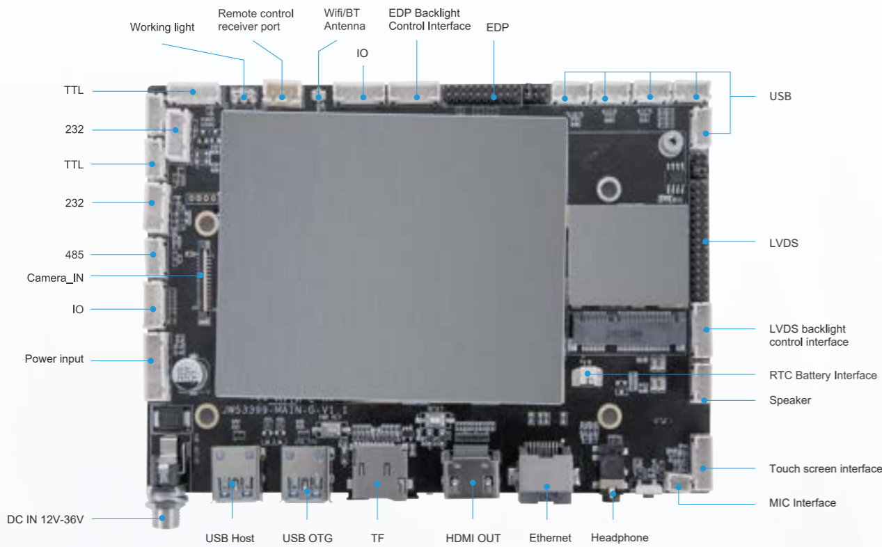
PCB: 6-layer board, size: 154*106mm, board thickness 1.6mm, screw hole specification: \phi 3.2mm x4
