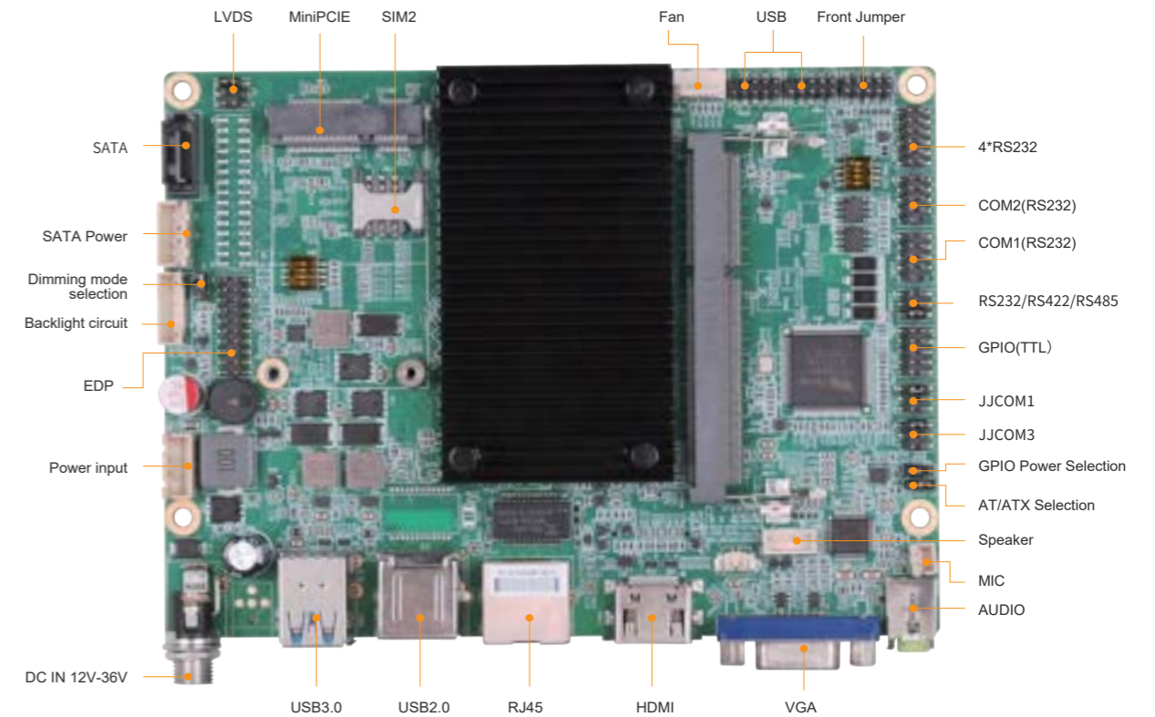
PCB: 8-layer board, size: 150*110mm, board thickness 1.6mm, screw hole specification: \phi 3.2mm x4
