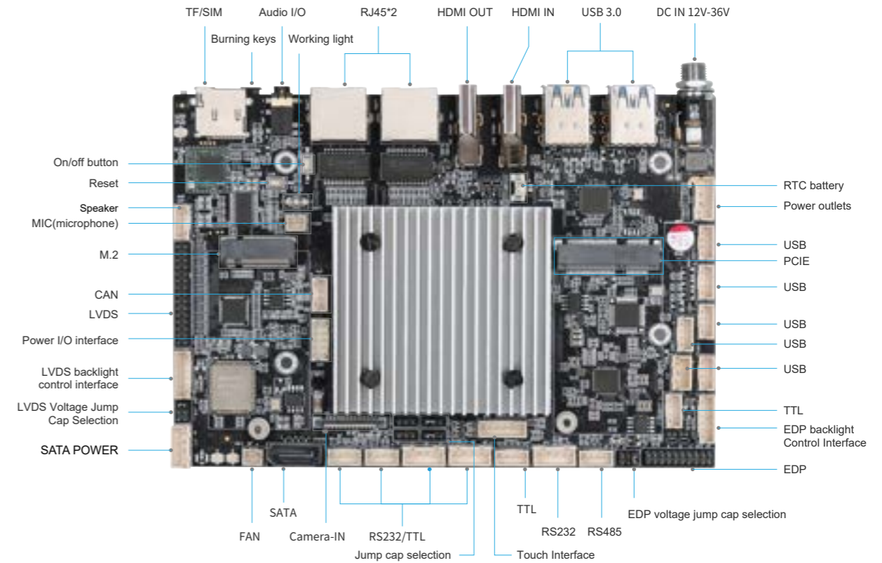
PCB: 6-layer board, size: 160*109mm, board thickness 1.6mm, screw hole specification: \phi 3.2mm x4
