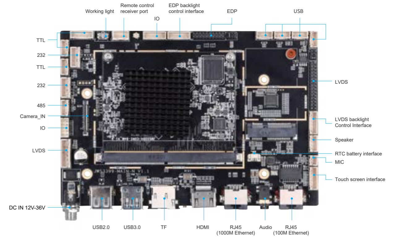
PCB: 6-layer board, size: 160*109mm, board thickness 1.6mm, screw hole specification: \phi 3.2mm x4
