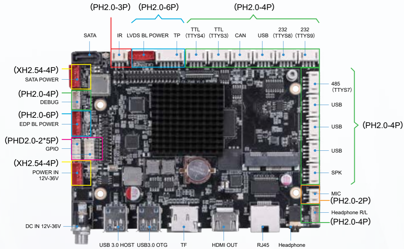
PCB: 6-layer board, size: 140*100mm, board thickness 1.6mm, screw hole specification: \phi 3.2mm x4
