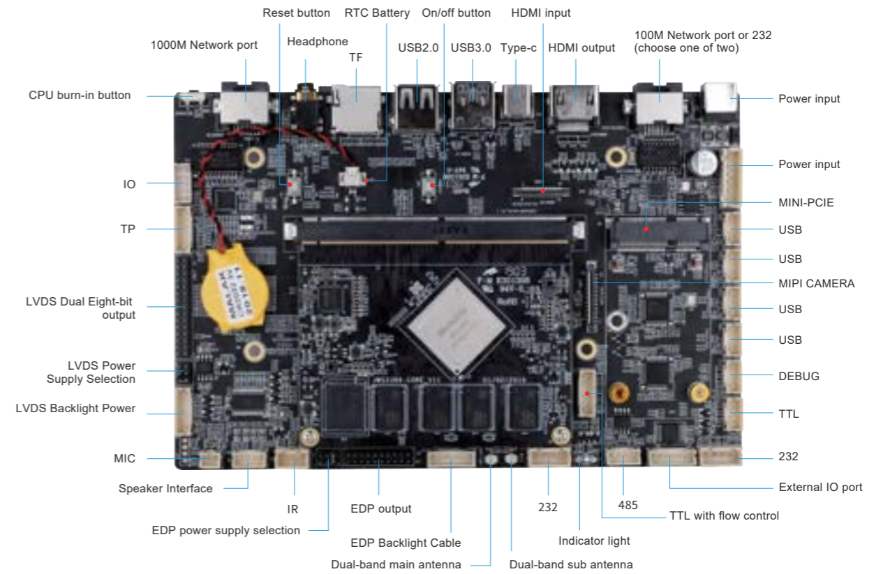
PCB: 10-layer board, size: 151.9*106mm, board thickness 1.6mm, screw hole specification: \phi 3.2mm x4
