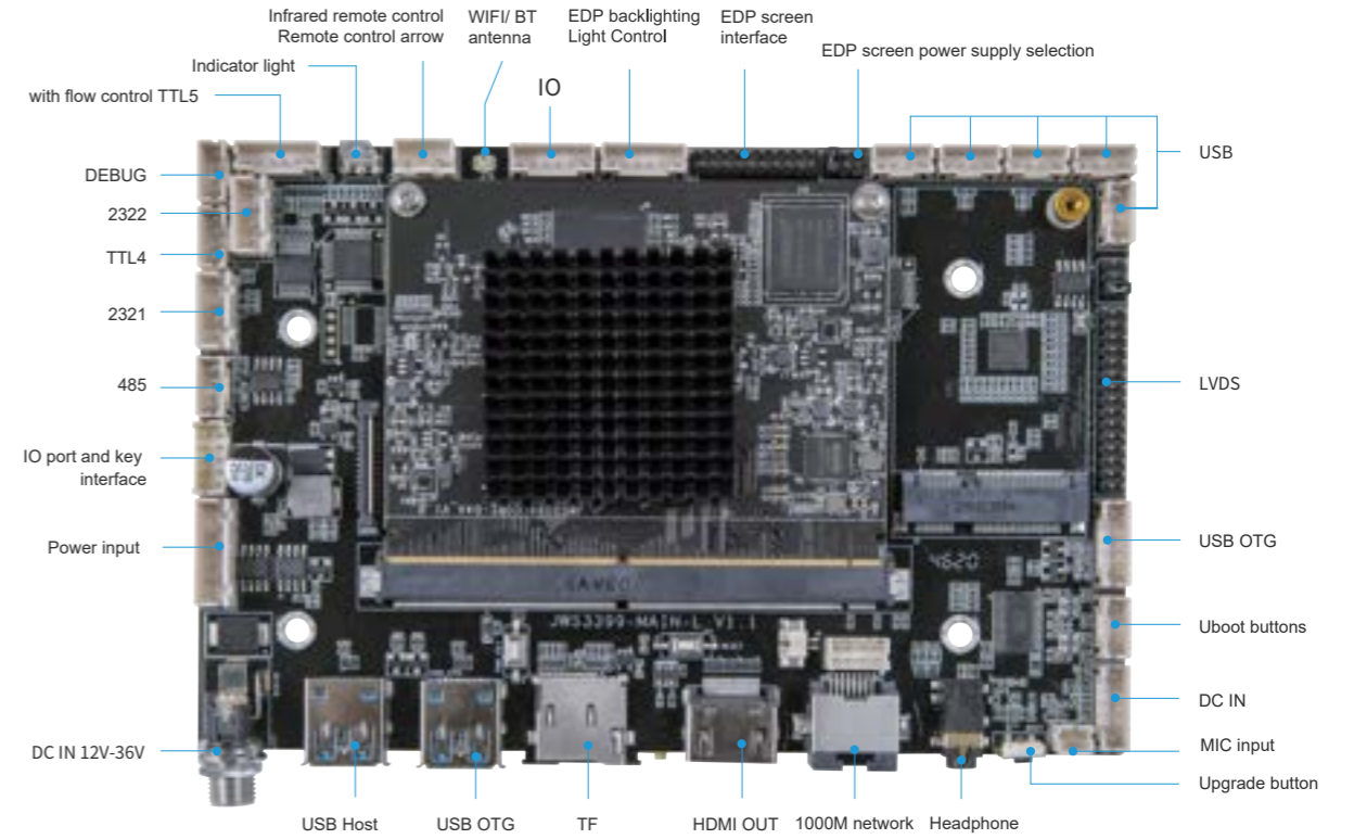
PCB: 4-layer board, size: 153.77*100mm, board thickness 1.6mm, screw hole specification: \varnothing 3.2mm x4
