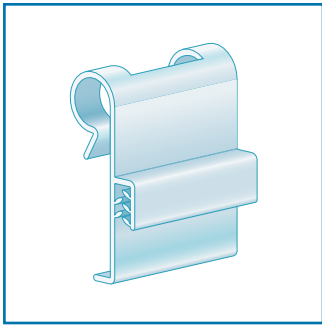
Fence & Basket Clip-On, Flush Grip with Double Loop (94FG)
