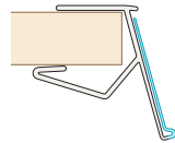
76WT — Thick Shelf, 15° Angle
