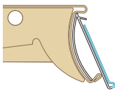
35LC — C-Channel (fits a variety of clip-in applications)
