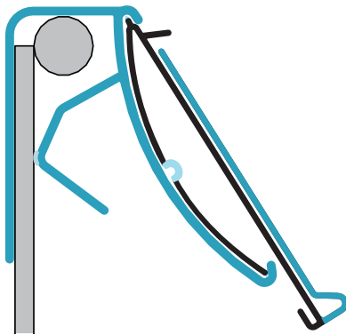
275A FlexKlip® Fence Adapter combined with 278T ClearVision® FlexChannel® Ticket Molding.
