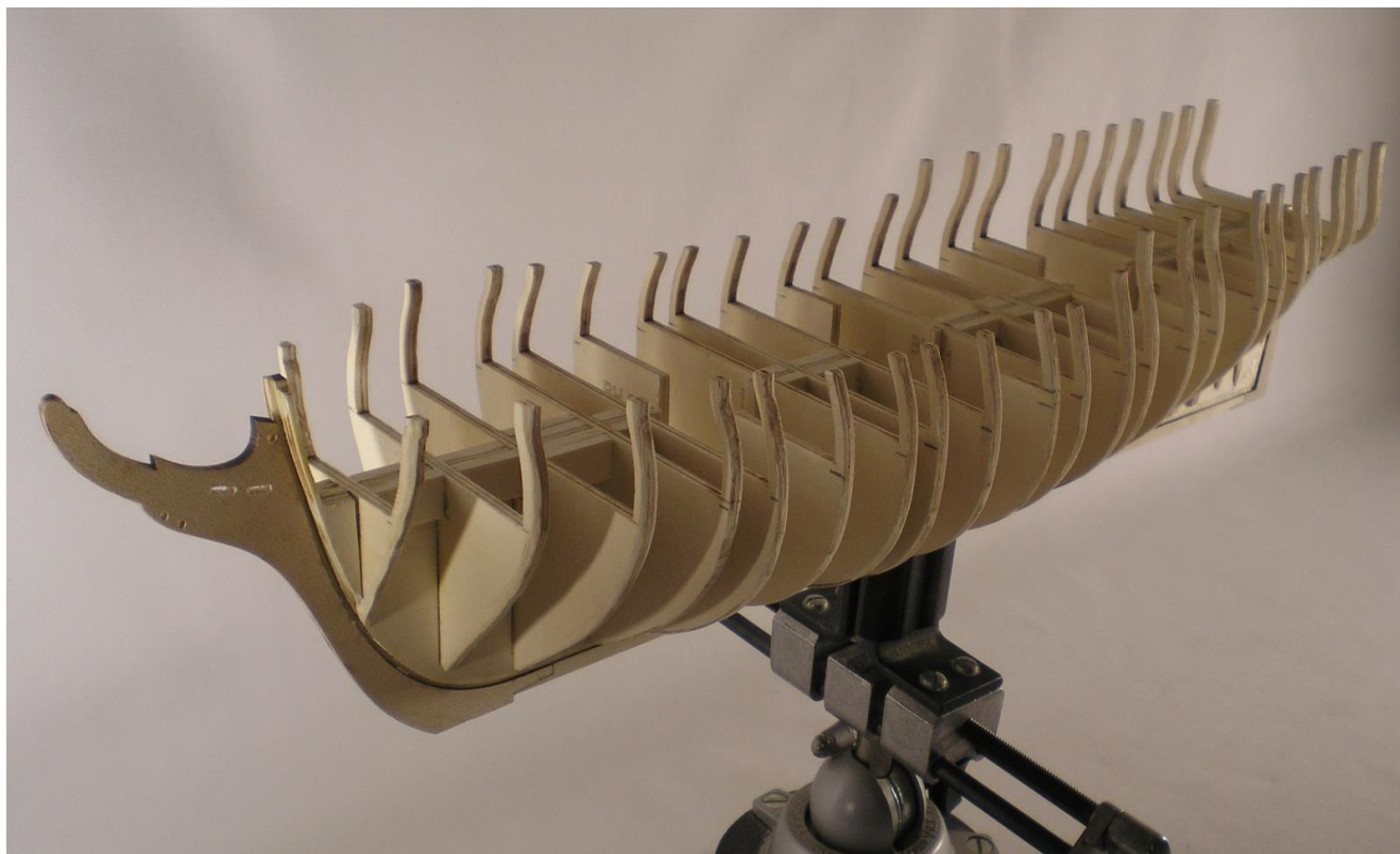
Fig 2c Note: Filler blocks installed along Former
