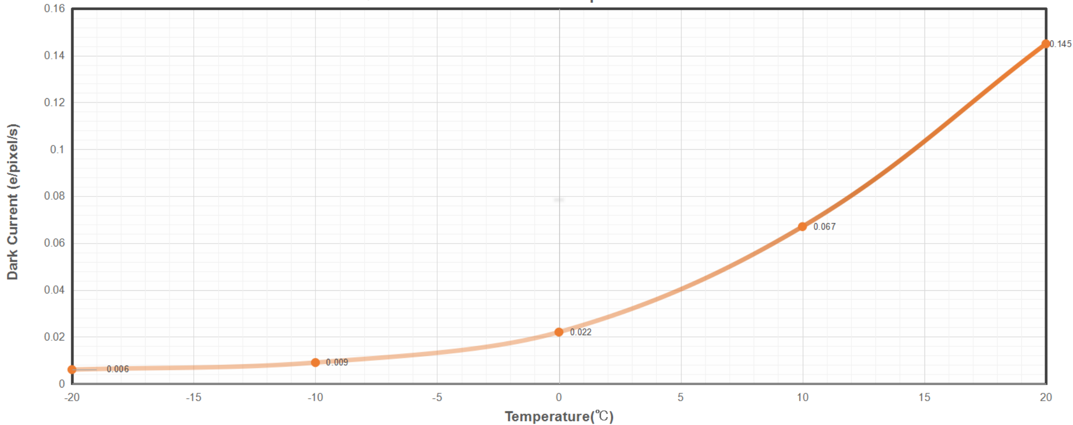
QHY163 Dark Current VS. Temperature
