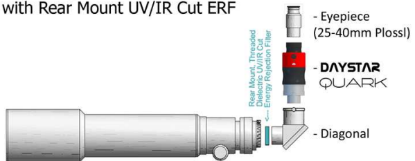
Daystar Quark Configuration on Refractor with Rear Mount UV/IR Cut ERF
