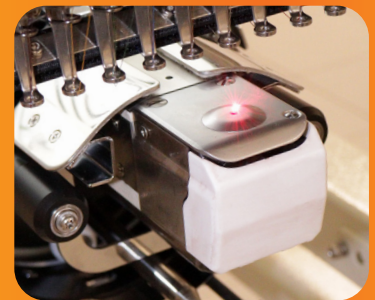
Centering laser
