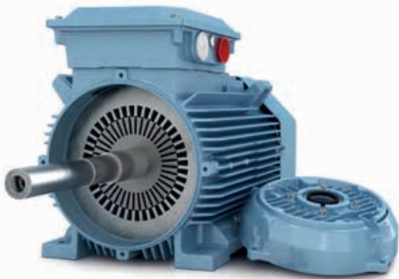
Traditional IE2 induction motor
