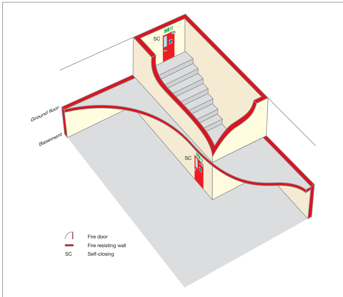
Figure 33: Basement protection
