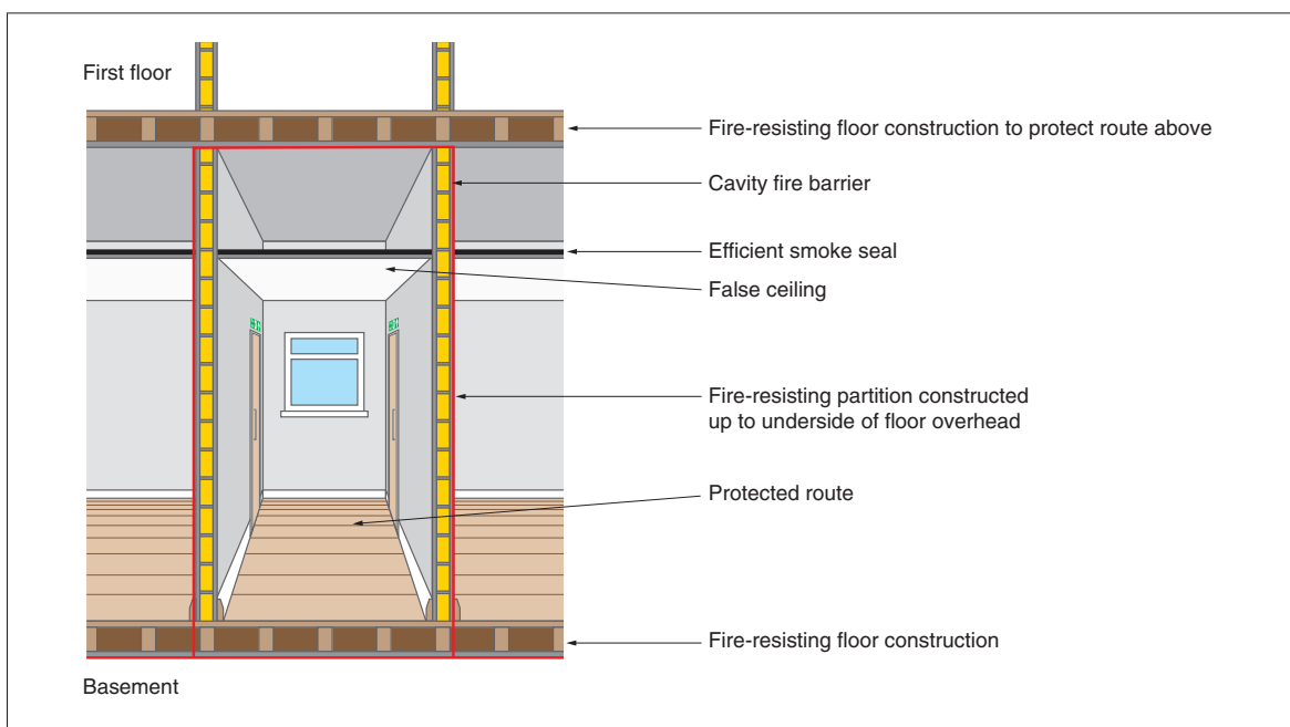
Figure 62: Fire-resisting construction
