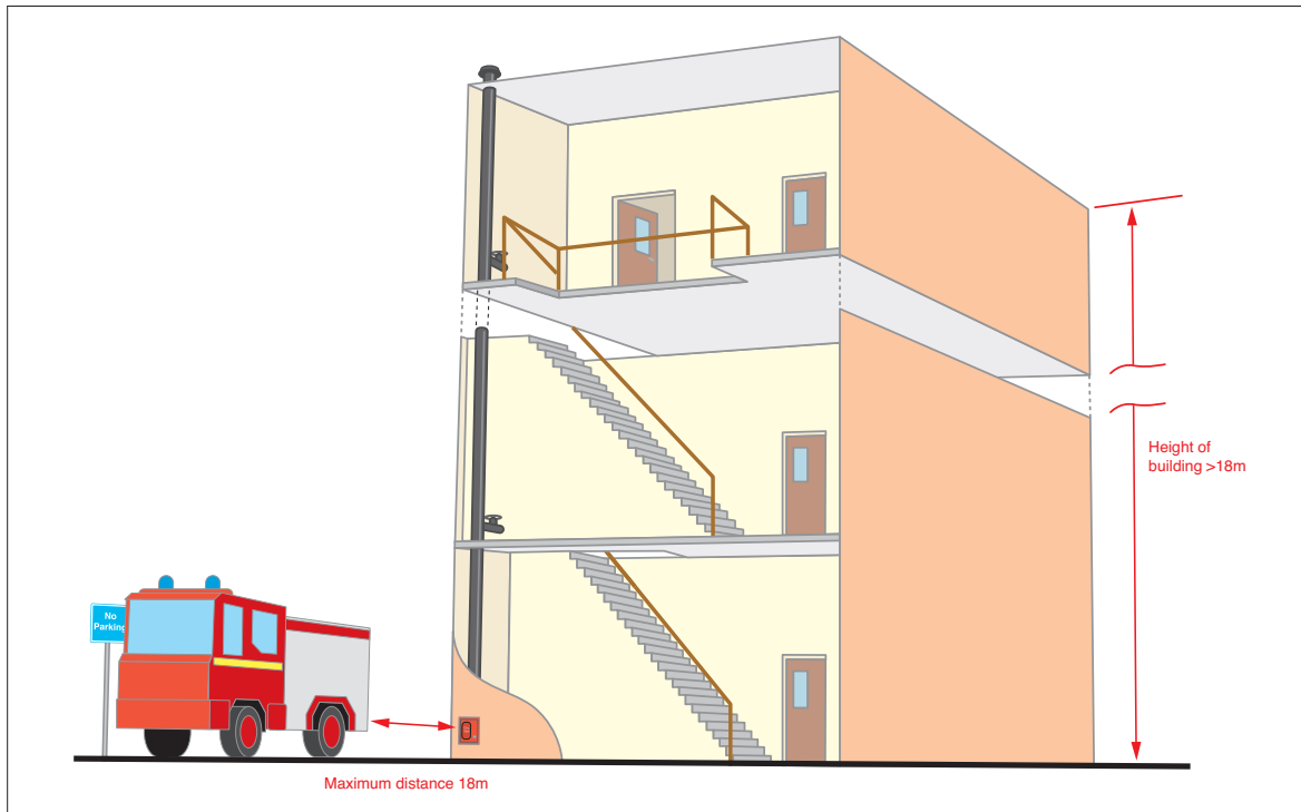
Figure 22: Rising main
