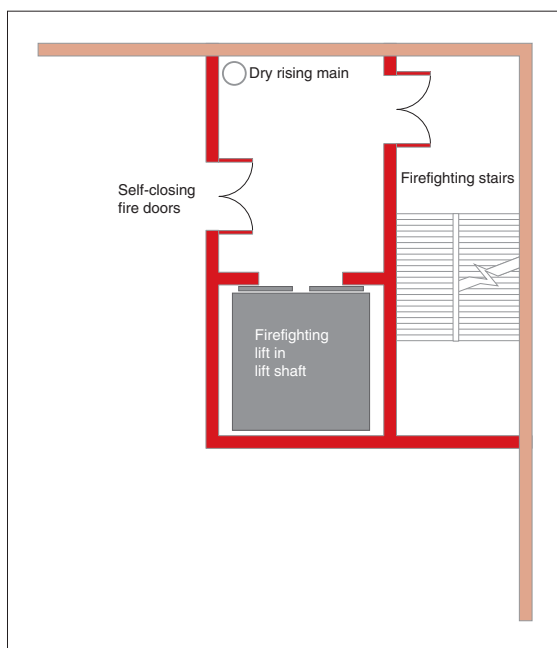
Figure 21: Firefighting shaft
