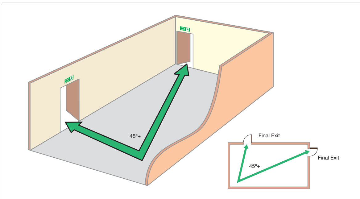
Figure 26: Alternative exits
