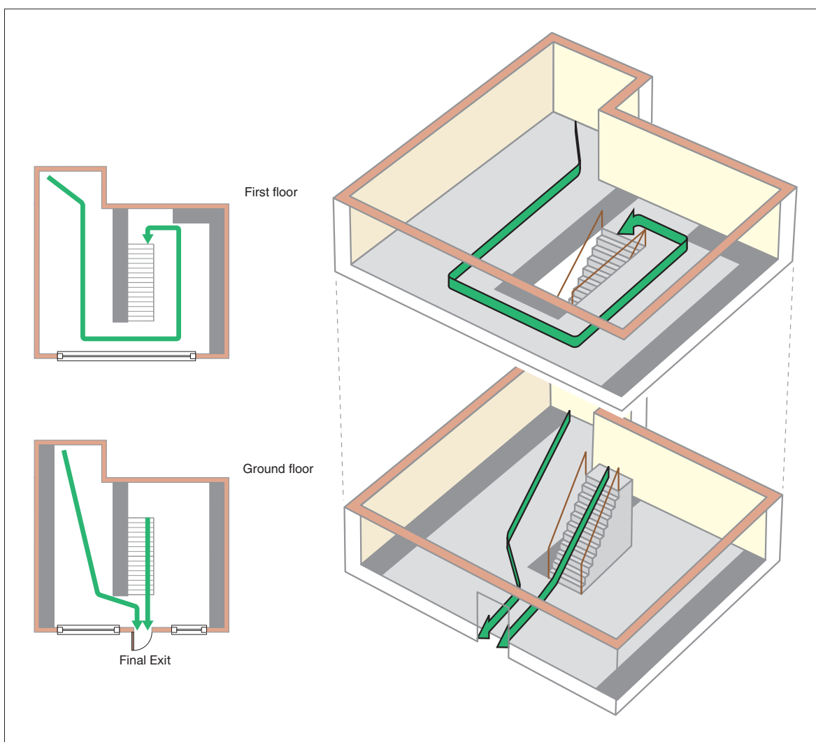
Figure 45: Two-storey premises
