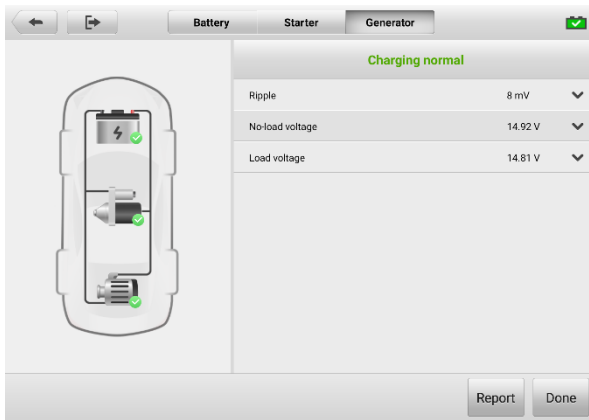
Figure 11-8 Generator Test Results Screen
