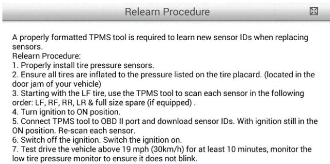
Figure 6-29 Sample OBDII Relearn Screen 2
