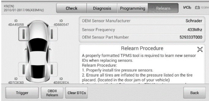
Figure 6-28 Sample OBDII Relearn Screen 1
