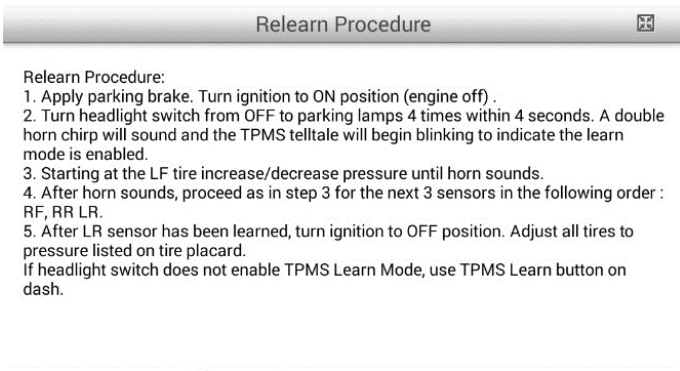
Figure 6-25 Sample Stationary Relearn Screen 2
