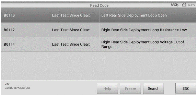
Figure 6-12 Sample DTCs Screen
