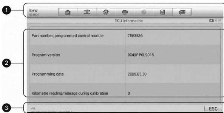
Figure 4-11 Sample ECU Information Screen
