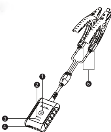
Figure 7-1 MaxiBAS BT506 Tester
