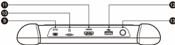
Figure 2-3 MaxiCheck MX808TS, Top View
