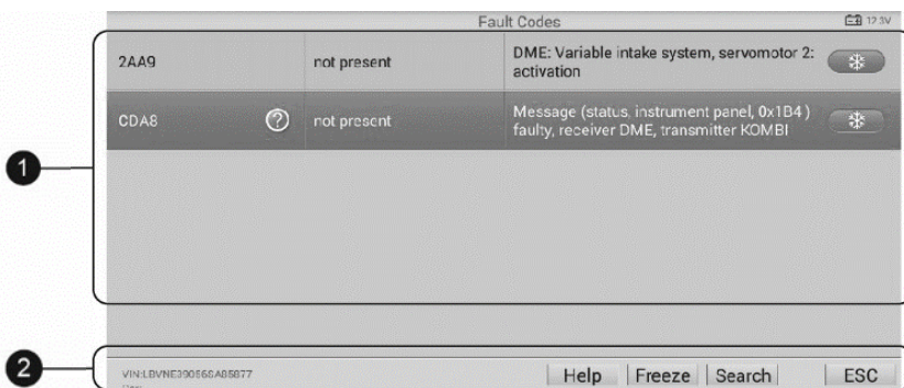
Figure 4-12 Sample Read Codes Screen
