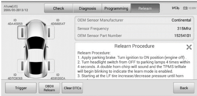
Figure 6-24 Sample Stationary Relearn Screen 1
