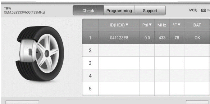
Figure 6-33 Sample Check Screen via OEM Part No.
