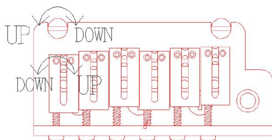
Modern Two-Point Synchronized Tremolo
