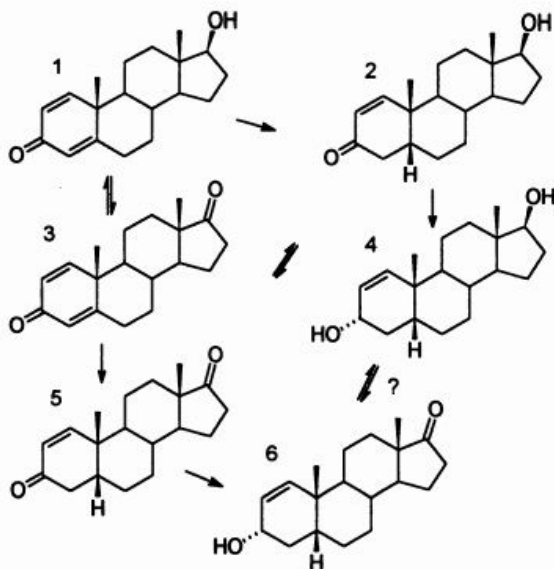
Fig. 11. Metabolism of boldenone (1) to 17β-hydroxy-5β-androst-1-en-3-one (2); androsta-1,4-diene-3,17-dione (3; intermediate, not excreted into urine); 5β-androst-1-ene-3α,17β-diol (4); 5β-androst-1-ene-3,17-dione (5; intermediate, not excreted into urine); and 3α-hydroxy-5β-androst-1-en-17-one (6).
