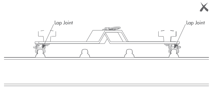
DWG 8 - Incorrect Clamp Placement (Off roof sheet lap joint)
