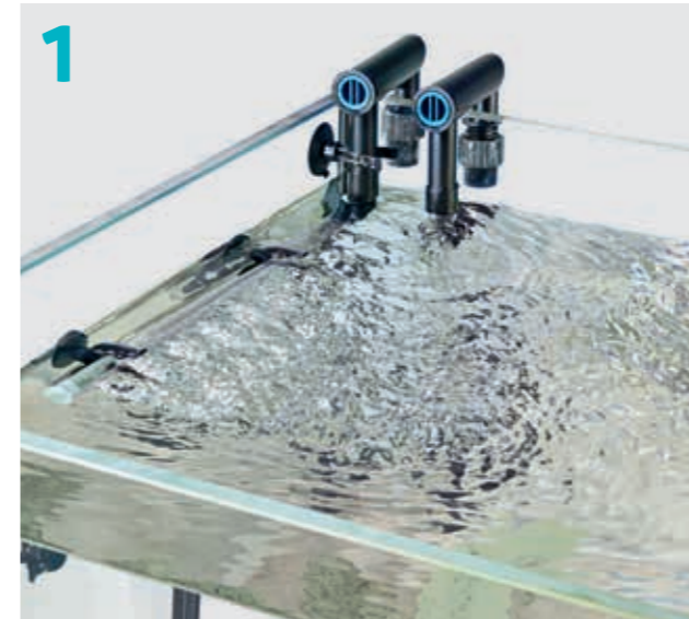
1. Complete quick start set: Includes filter media, hoses, adapters, flow regulator, suction and discharge pipe as well as water diffuser
