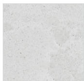
Glacier (Quartz)
