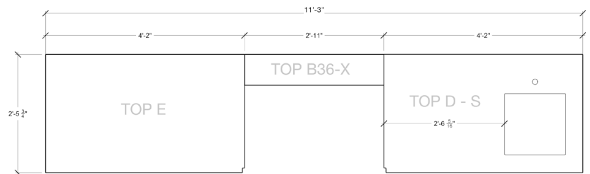
COUNTERTOP TEMPLATE
