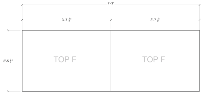
TOP VIEW (Gas & Electrical Conduits Access Points)
