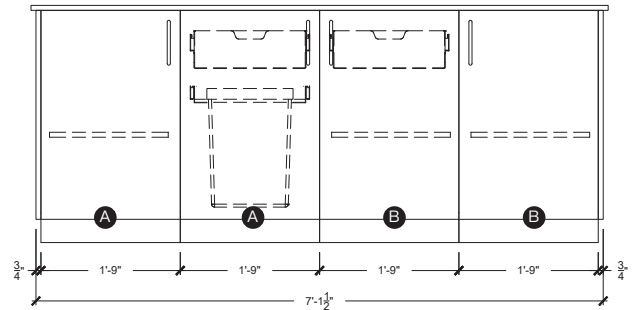
COUNTERTOP TEMPLATE
