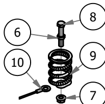
034-8045-04 Seat Spring Assembly w/Cable
