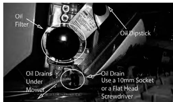
Parts Location
