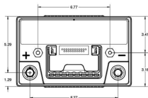
ODX-AGM34M LEFT POSITIVE DUAL TERMINALS (SAE & STUD)
