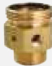
3-1/4" EXTENDED ACME ADAPTER W/ INTEGRATED RELIEF & BLOWDOWN PORTS
