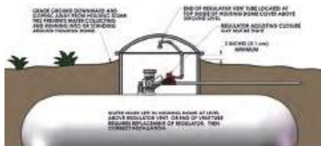
Figure 5: Underground installation
