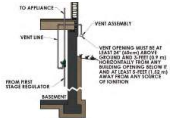
Figure 4: Basement installation
