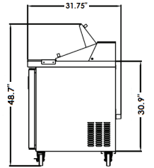
Side View of all Sandwich Prep Tables
