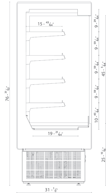
Optional Mounting
