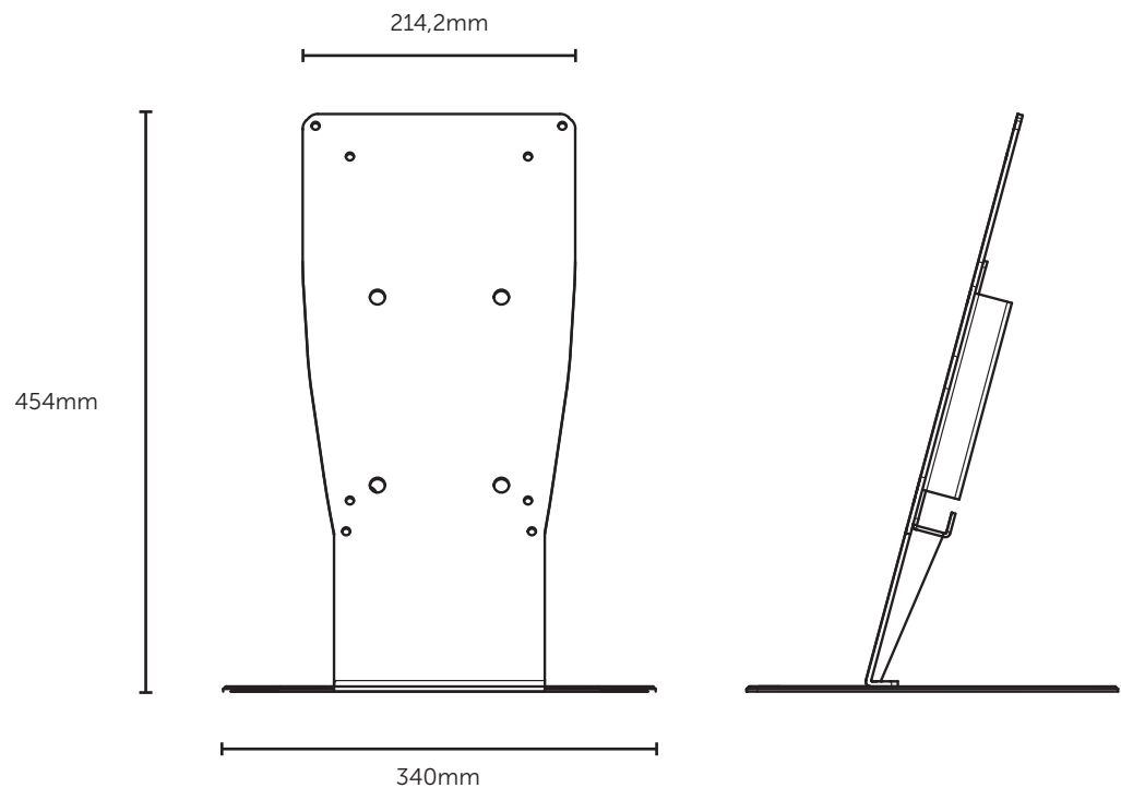
Technical drawing
