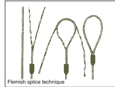
Sling with Single Part Body
