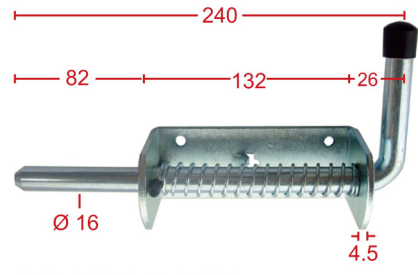
SPRING BOLT HEAVY DUTY LARGE
