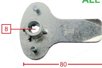
LATCH LEG PRESSED METAL • Multiple Position Hole
