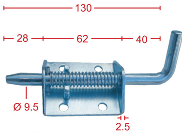
SPRING BOLT HEAVY DUTY SMALL
