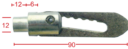
ANTI-LOOSE FASTENER WELD ON SH-036A Zinc
