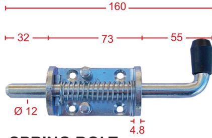
SPRING BOLT HEAVY DUTY MEDIUM
