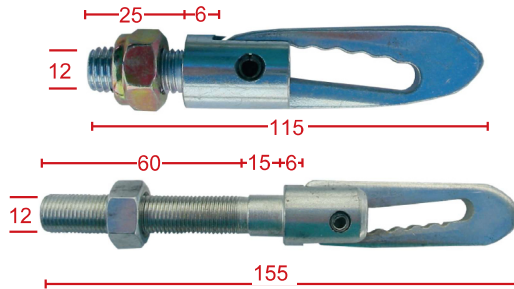
ANTI-LOOSE FASTENER BOLT ON SH-036B Zinc 25mm Thread SH-036C Zinc 60mm Thread
