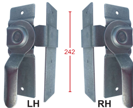
CORNER FASTENER BOLT - ON SH-034SET FULL SET 2 X LH Latch & Catch 2 X RH Latch & Catch SH-034LH 1 X LH Latch & Catch Only SH-034RH 1 X RH Latch & Catch Only
