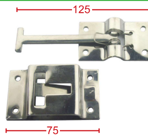
DOOR HOLD - T HOOK STYLE HEAVY DUTY • Holder incorporates retaining spring SH-040 Stainless steel
