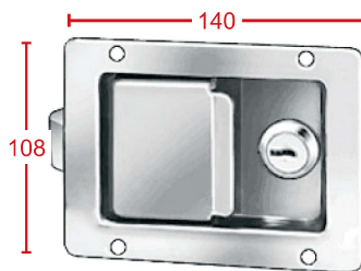
SLAM LATCH KEY LOCKING FLUSH MOUNT • Large Size
