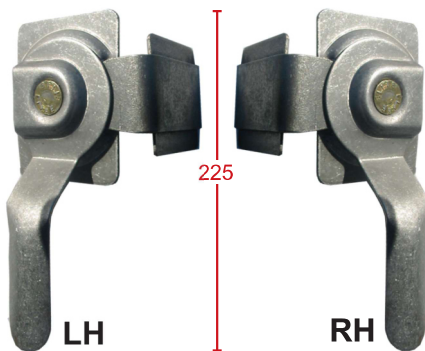
CORNER FASTENER WELD - ON SH-033SET FULL SET 2 X LH Latch & Catch 2 X RH Latch & Catch SH-033LH 1 X LH Latch & Catch Only SH-033RH 1 X RH Latch & Catch Only
