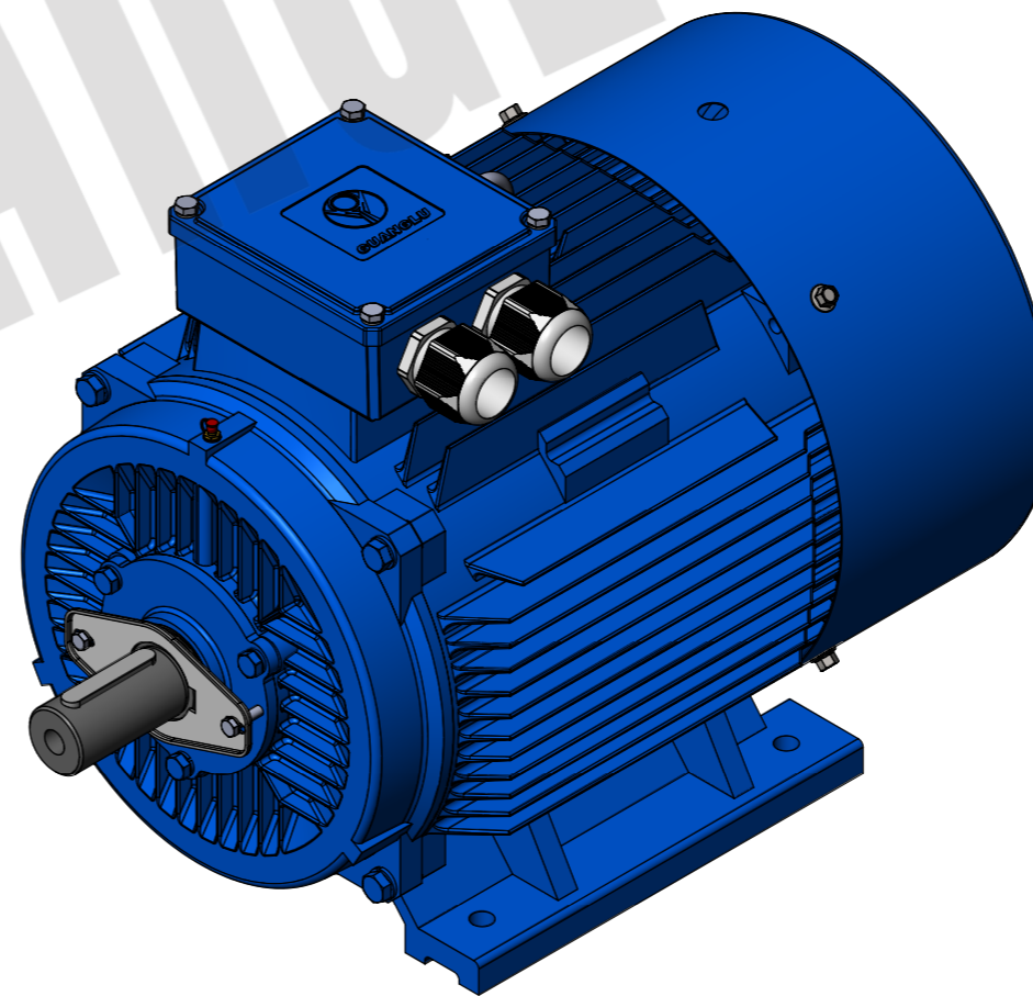
YX3-225M-B3-2 Mounting diagram
