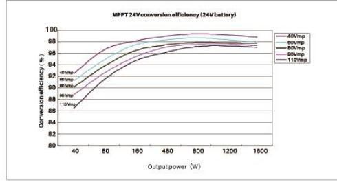
-7.1 24V System Conversion Efficiency
