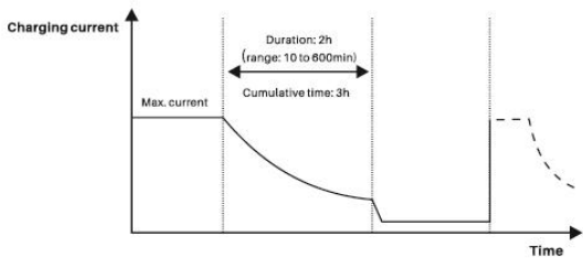
Fig. 1-5 SLD Battery charging stages diagram
