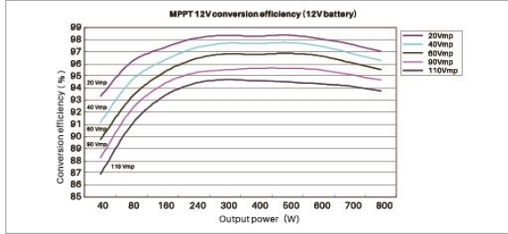
-7.1 12V System Conversion Efficiency
