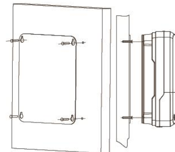
Fig. 2.1 Installation and heat dissipation
