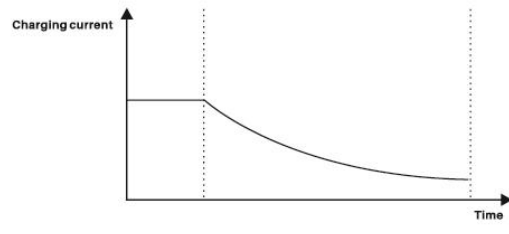
Fig. 1-6 LI Battery charging stages diagram
