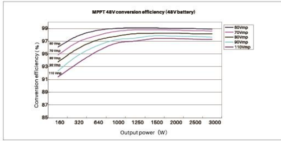
-7.3 48V System Conversion Efficiency
